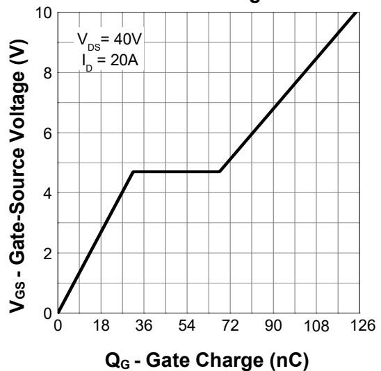
Gate Charge
