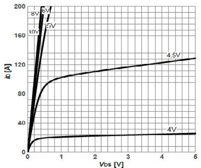
Diagram12: Typ. output characteristics
