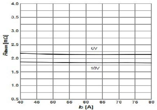
Diagram10: On-state resistance vs. Drain current
