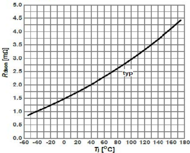
Diagram 5: On-state resistance vs. Junction temperature
