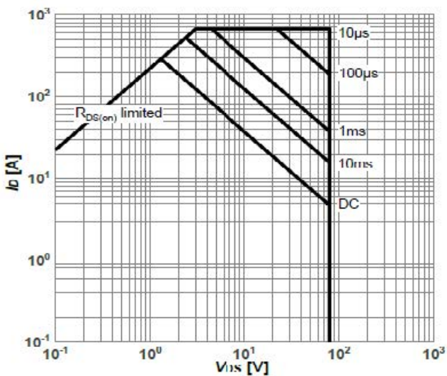
Diagram11: Safe operating area
