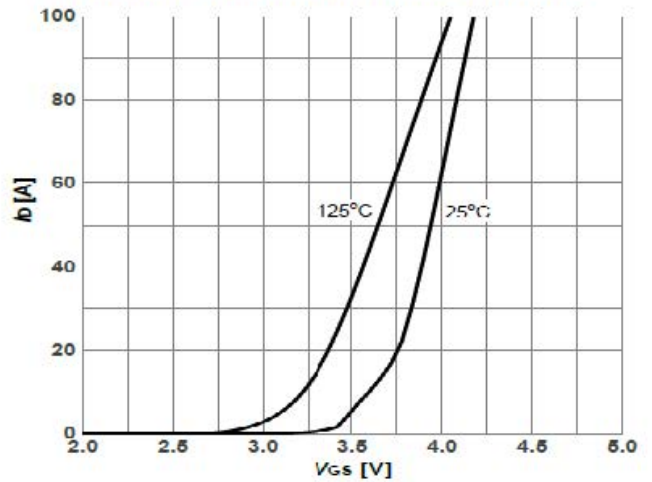
Diagram 4: Typ. transfer characteristics
